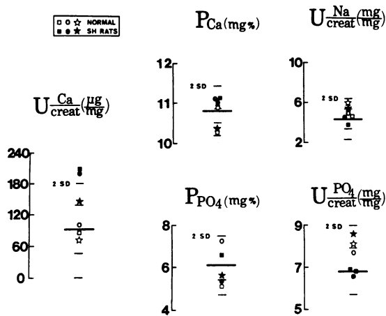
FIGURE 1 Biochemical profile of the parental generation (n = 24) from which three female hypercalciuric (solid symbols) and three female normocalciuric rats (open symbols) were identified and chosen as breeders. Heavy horizontal bars represent the mean of the group of 24 rats and lighter bars SD of the mean. U, urine; P, plasma. Only plasma PO 4 was obtained after 12-h fast.
