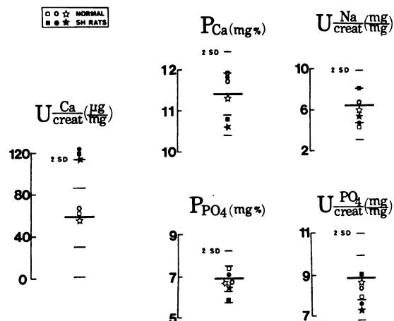
FIGURE 2 Biochemical profile of the male parental generation (n = 24) from which three hypercalciuric (solid symbols) and three normocalciuric rats (open symbols) were identified and chosen as breeders. Abbreviations and symbols are as defined in Fig. 1.
