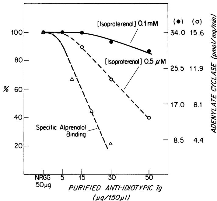
FIGURE 2 The effects of DEAE-purified Ig fraction on (-)-[^3\text{H}]\text{alprenolol} (2 nM) binding to turkey erythrocyte membranes and on isoproterenol-mediated adenylate cyclase stimulation were assessed. The Ig fraction was purified on DEAE-cellulose as described in Methods. The Ig fraction was then dialyzed into 100 mM Tris, pH 7.4. The ability of the antiidiotypic Ig fraction to inhibit adenylate cyclase stimulation in the turkey erythrocyte membrane was tested at isoproterenol concentrations of 0.5 \mu\text{M} and 0.1 mM in the presence of 0.1 mM GTP. In contrast to the effects seen at the nonsaturating isoproterenol concentration of 0.5 \mu\text{M} , only a slight amount of inhibition is seen at the highest Ig concentrations in the presence of 0.1 mM isoproterenol. NRGG, normal rabbit gamma globulin.
