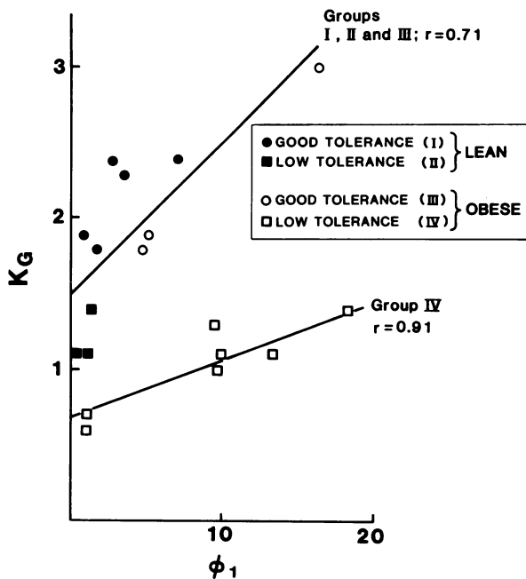
FIGURE 6 Dependence of K_G upon \phi_1 in subjects from groups I, II, and III (upper line, n = 11 , S_1 = 5.1 \pm 0.7 \text{ min}^{-1} / \mu\text{U per ml} ) and group IV (lower line, n = 7 , S_1 = 2.0 \pm 0.4 \text{ min}^{-1} / \mu\text{U per ml} ). Insulin resistance was characteristic of group IV, but not I, II and III (Table III). Slopes of the two lines are significantly different ( P < 0.01 ).
