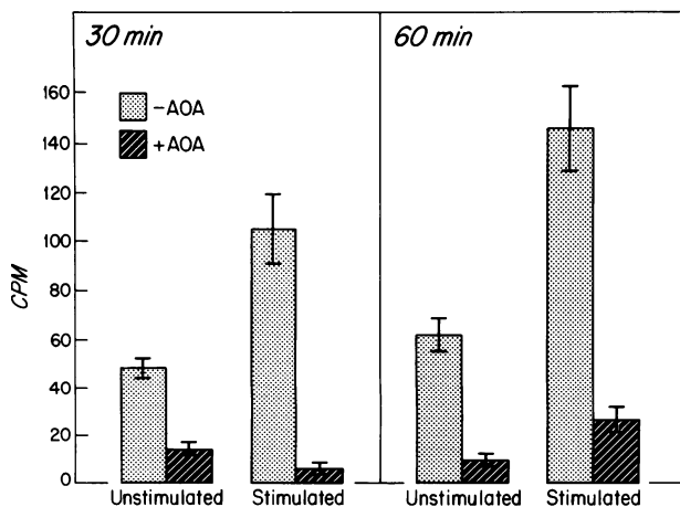
FIGURE 5 Effect of amino-oxoacetate on ^{14}\text{CO}_2 production from L-[1- ^{14}\text{C} ]alanine (1 mM) by resting and phagocytizing PMN at two time intervals. For details see Methods.
