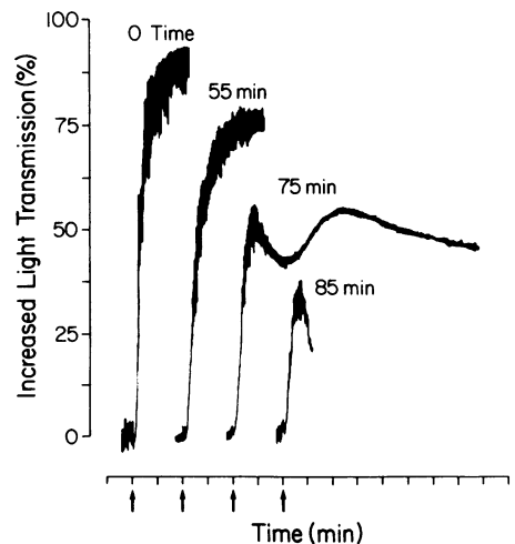
FIGURE 2 Human platelet responsiveness to AGEPC at various times after PRP preparation. The numbers above the aggregation curves indicate the time after citrated PRP preparation at which the aggregation assays were performed. The final molar concentration of AGEPC was 0.2 μM.
