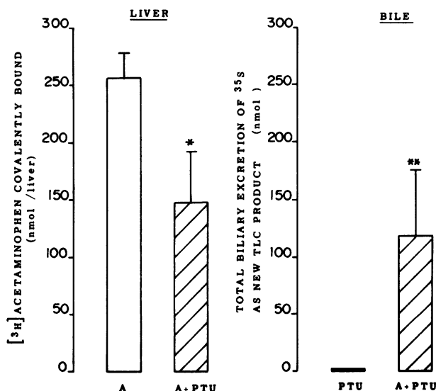
FIGURE 7 Comparison of PTU induced inhibition of total [ 3 H]acetaminophen covalently bound to rat whole liver homogenates vs. total biliary excretion of [ 35 S]PTU product as defined and separated by thin layer chromatography (TLC). Two groups of 10 phenobarbital pretreated rats each were administered 0 or 150 mg [ 35 S]PTU(P). 30 min later, the groups were each divided into two subgroups of five rats and treated with 0 or 750 mg/kg [ 3 H]acetaminophen (A). Bile was collected from each rat for 4 h, after which the animals were killed and their whole liver homogenates were assayed for [ 3 H]acetaminophen covalent binding. Bile samples were applied to thin layer chromatography as noted in Fig. 6 and the total amount of 35 S eluting as new product was counted. Results are depicted as mean \pm SE. The reduction in covalent binding resulting from PTU treatment (108 nmol), which is the difference between the two bars on the left, approximates total biliary excretion of new [ 35 S]PTU product (116 nmol). This product was not found in rats treated with PTU alone. * P < 0.05 ; ** P < 0.001 .
