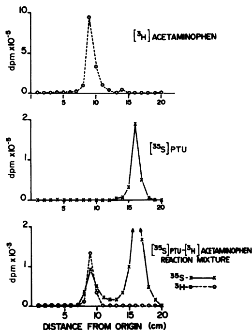
FIGURE 6 Thin layer chromatography of [ ^3\text{H} ]acetaminophen, [ ^{35}\text{S} ]PTU, and [ ^{35}\text{S} ]PTU-[ ^3\text{H} ]acetaminophen reaction mixture using a chloroform/benzene/methanol (3:1:1) solvent system for elution. Sections (1 cm) were scraped from the 20 \times 20 plates, eluted with hot water, and counted for ^3\text{H} , ^{35}\text{S} , or both. A new ^{35}\text{S} peak could be separated in the reaction mixture that was separate from the [ ^{35}\text{S} ]PTU peak but that coeluted with the [ ^3\text{H} ]acetaminophen peak.
