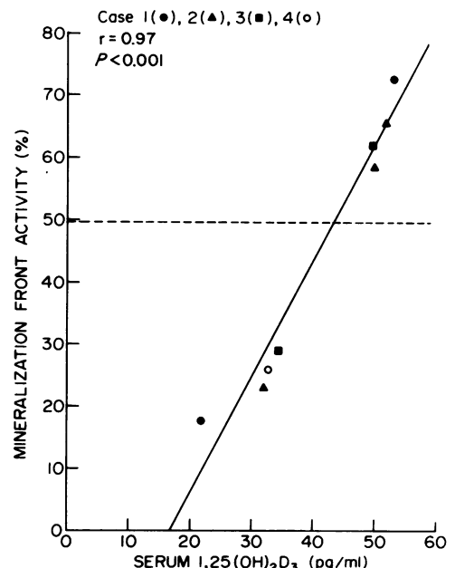
FIGURE 3 Correlation between the mineralization front activity in bone biopsies and the circulating concentration of 1,25(\text{OH})_2\text{D}_3 . Bone biopsies were obtained (and mineralization front activity determined) in the four subjects studied in the base-line period, after 6 mo of therapy with 1,25(\text{OH})_2\text{D}_3 in the three treated subjects (while on 3.00 , 2.50 , and 2.25 \mu\text{g}/\text{d} , respectively) and after 12 mo of therapy in cases (while on 2.75 \mu\text{g}/\text{d} ) 1, 2, and 3. Serum 1,25(\text{OH})_2\text{D}_3 levels were determined at 11 a.m. on the 2 d preceding bone biopsy in each case as described in Methods. Because the 6- and 12-mo biopsies in case 2 were performed on different doses of medication both points are displayed. In contrast, the 6- and 12-mo biopsies on case 1 and 3 were performed on the same dose of medication and are displayed as a single point, because no significant difference in mineralization front activity or 1,25(\text{OH})_2\text{D} serum levels were present. The dotted line represents the lower level of normal mineralization front activity. It is evident that a significant correlation exists between the measured parameters.
