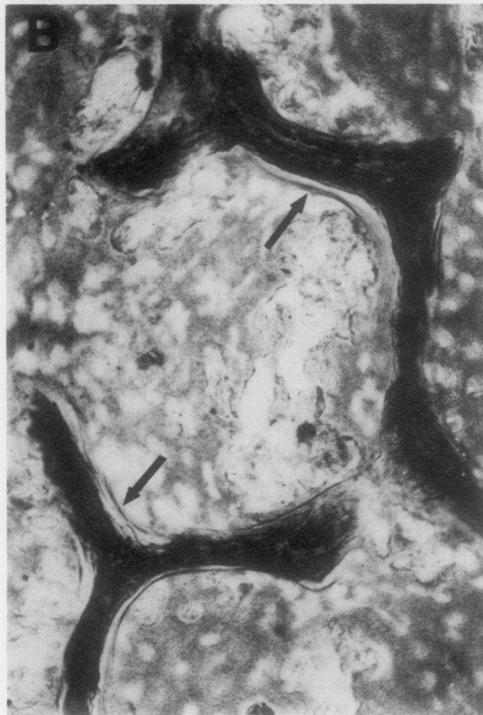
FIGURE 1 (A) Microradiograph showing both hypomineralized "splits" (S) and patchy osteocytic osteolysis (O). (B) Unstained section demonstrating extensive osteoid seams (arrows) with minimal mineralization.
