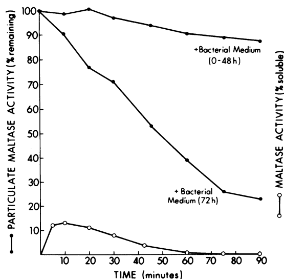
FIG. 2 The effect of bacterial medium on the maltase activity of human intestinal brush borders. Cell-free supernate medium was produced from B. thetaiotamicron , as described in Methods, after growth up to 48 h, and after 72 h. The equivalent of 10 \mu g of trypsin was added to 0.5 \mu g of brush border protein in a reaction mixture of 1.0 ml at pH 7.5. At times indicated, the reaction mixture was centrifuged at 40,000 g for 20 min, washed with 1 ml of buffer, recentrifuged, and the pellet resuspended by homogenization in 1 ml of 200 mM Na 2 PO 4 buffer, pH 7.5. Aliquots of the supernate and resuspended pellets were assayed for maltase activity in the presence of 5 mM EDTA and 1 mM PCMB to inhibit bacterial maltase. The points represent the mean of duplicate experiments. Control maltase activity (100%) corresponded to 0.72 OD at 420 \mu m.
