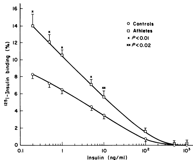
FIGURE 1 Specific binding of ^{125} I-insulin to monocytes in control subjects and athletes in the resting state. Mononuclear cells ( 4 \times 10^7 /ml) were incubated with ^{125} I-insulin (0.2 ng/ml) at 22^\circ\text{C} for 180 min in the absence (initial point of the curve) and presence of increasing concentrations of unlabeled insulin. Data are expressed per 1 \times 10^7 monocytes/ml.
