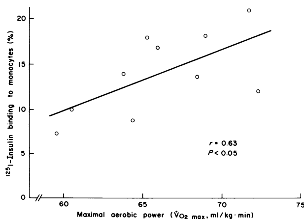
FIGURE 2 The relationship between specific ^{125} I-insulin binding to monocytes and \dot{V}O_{2\max} in athletes in the resting state.
