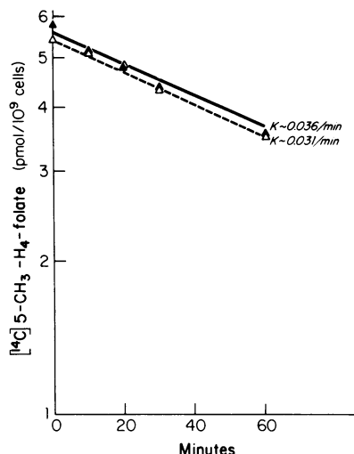
FIGURE 8 Release of [ ^{14}\text{C} ]5-CH 3 -H 4 -folate from control and energy-depleted cells. When loaded with approximately equal amounts of radioisotope, as described in the text, rate constants of efflux ( K ) from control ( \blacktriangle — \blacktriangle ) and F/CN-treated ( \triangle --- \triangle ) cells are nearly identical. Each triangle represents the mean of six experiments, done in triplicate. Lines were fit by the method of least squares.
