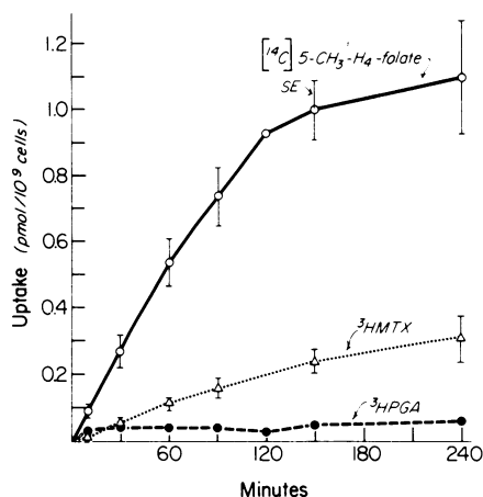
FIGURE 5 Comparative uptake of folate analogues by erythrocytes. Erythrocytes were incubated with 0.1 \mu M of [ ^{14} C]5-CH 3 -H 4 -folate (○ — ○), [ ^3 H]Mtx (△ — △), or [ ^3 H]PGA (● — ●). Each point is the mean of duplicate assays in three separate experiments utilizing different erythrocyte (RBC) suspensions; brackets represent SE of the mean.
