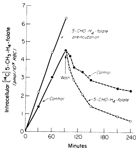
FIGURE 6 Stimulation of [ ^{14} C]5-CH 3 -H 4 -folate uptake and efflux by counter-transport. Uptake of [ ^{14} C]5-CH 3 -H 4 -folate is increased in erythrocytes incubated with 5-CHO-H 4 -folate (○ — ○) compared to control cells (● — ●). When cells containing [ ^{14} C]5-CH 3 -H 4 -folate were washed (↑) and resuspended in folate-free PBS (● — ●) or PBS containing 5-CHO-H 4 -folate (○ — ○), efflux of radioactivity was enhanced by the presence of 5-CHO-H 4 -folate.
