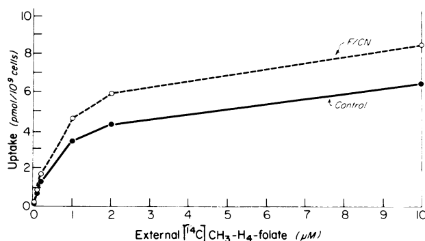
FIGURE 7 Effect of erythrocyte ATP depletion on [ ^{14} C]5-CH 3 -H 4 -folate uptake. Erythrocytes after 4 h in PBS (● — ●) or in PBS plus 10 mM sodium fluoride/4 mM sodium cyanide (○ — ○) were washed, then incubated for 90 min with increasing concentrations of [ ^{14} C]5-CH 3 -H 4 -folate. Each point represents the mean of six experiments. The difference between uptake by control and F/CN-treated cells is statistically significant at all concentrations tested.
