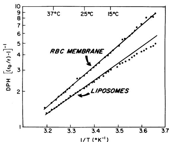
FIGURE 2 Temperature dependence of the fluorescence polarization of diphenylhexatriene in human erythrocyte (RBC) ghost membranes and in liposomes prepared from ghost membrane lipid. The horizontal axis is the reciprocal of the absolute temperature, with T = absolute temperature \times 10^{-3} .
