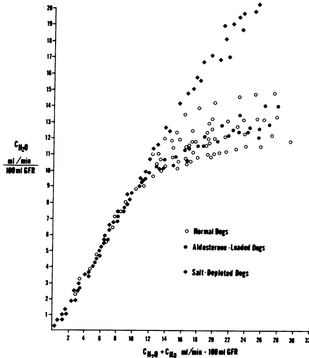
FIGURE 2 Comparison of the relationship between solute-free water clearance ( C_{H_2O} ) and sodium supply to the diluting segment ( C_{H_2O} + C_{Na} ) in normal ( n=7 ), salt-depleted ( n=6 ), and aldosterone-loaded normal dogs ( n=3 ) during hypotonic saline infusion.
