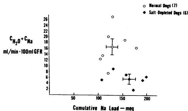
FIGURE 1 Comparison of the relationship between sodium supply to the diluting segment ( CH_2O + C_{Na} ) and cumulative sodium load in normal dogs and salt-depleted dogs during the steady-state water diuresis. The mean for each group is shown \pm 1 SEM for both CH_2O + C_{Na} and cumulative sodium load.
