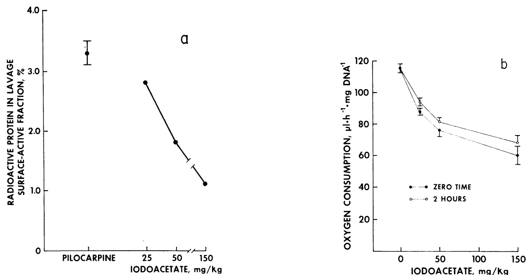
FIGURE 2 Influence of iodoacetate on lung \dot{Q}O_2 and pilocarpine induced secretion. a . These studies were performed as in Fig. 1 except that some rabbits received iodoacetate before the administration of pilocarpine but after the pulse-labeling procedure. The animals were sacrificed 2 h after administration of [ ^{14}\text{C} ]leucine. In the iodoacetate-treated animals each point is the mean of two animals. The other value is the mean \pm SEM of four rabbits. b . Rabbits were given the indicated amount of iodoacetate or an equal volume of saline i.p. They were then sacrificed immediately ( \bullet — \bullet ) or after 2 h ( \circ — \circ ) and the \dot{Q}O_2 of lung slices was measured. Mean \pm SEM are given.
