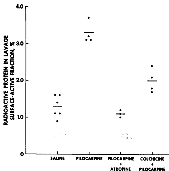
FIGURE 1 Stimulation and inhibition of protein secretion. L-[U- ^{14} C]leucine was given intravenously, followed in 4 min by a chase dose of nonradioactive leucine. The rabbits were given two injections of saline or pilocarpine i.p., 30 min apart, or two i.p. injections of pilocarpine 30 min apart each followed immediately by an i.v. injection of atropine, or one i.v. injection of colchicine 16 h before the administration of [ ^{14} C]leucine and subsequent i.p. injections of pilocarpine. The animals were sacrificed 2 h after the administration of L-[ ^{14} C]leucine. Each point represents one animal and the horizontal line indicates the group mean.
