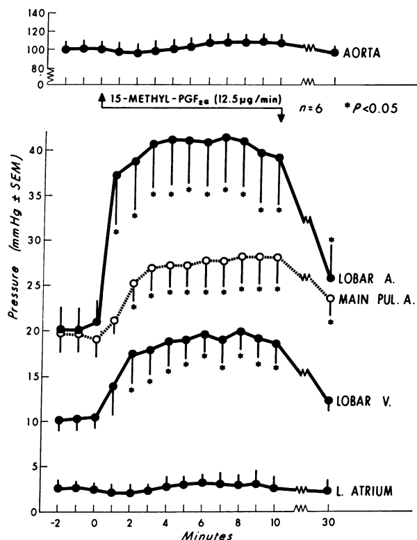
FIGURE 2 Effects of infusion of 15-methyl-PGF 2α , 12.5 \mu\text{g}/\text{min} , into the lobar artery on mean vascular pressures in the lobar artery, small intrapulmonary lobar vein, left atrium, the aorta, and main pulmonary artery. n indicates number of dogs studied.
