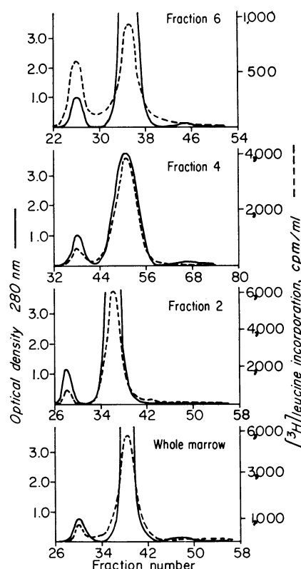
FIGURE 8 Gel filtration of the fractionated marrow lysates from a normal individual, W. S., showing the virtual absence of a free \alpha chain peak in any of the fractions.
