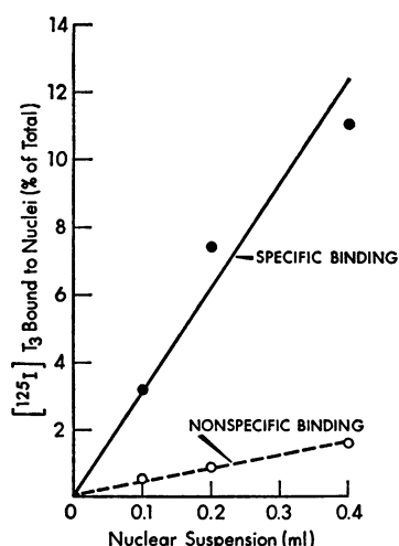
FIGURE 4 Linear relationship between specific [ ^{125}\text{I} ]T 3 binding to isolated nuclei and the concentration of nuclei incubated. [ ^{125}\text{I} ]T 3 incubated as per the legend to Fig. 3 with an increasing concentration of hepatic nuclei (from 0.1 to 0.4 ml suspension of isolated nuclei) equivalent to nuclei harvested from 0.1 to 0.4 g liver in 1 ml incubation medium. Specific nuclear binding is proportional to the nuclear concentration.
