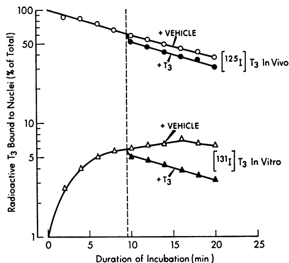
FIGURE 5 Similar rate of release for T 3 bound to specific nuclear sites in vitro and for endogenous nuclear T 3 upon incubation of isolated nuclei in vitro. Endogenous nuclear T 3 was labeled by injection of [ ^{125}\text{I} ]T 3 (5 ng/100 g body weight) 30 min before the rats were killed and the liver nuclei harvested. The nuclear suspensions were then incubated in vitro for 10 min with [ ^{125}\text{I} ]T 3 (1 pmol/ml) and a loading dose of T 3 (not illustrated). Samples were withdrawn at the indicated time intervals to determine the percent of in vitro-bound [ ^{125}\text{I} ]T 3 (open triangles) and endogenous [ ^{125}\text{I} ]T 3 (open circles) bound to specific nuclear sites. At 9.5 min of incubation (vertical interrupted line) the incubation mixture was divided. Nonradioactive T 3 (3,000 pmol/ml) was added to one portion (filled circles or triangles) to prevent reuptake by nuclei of [ ^{125}\text{I} ]T 3 or [ ^{125}\text{I} ]T 3 from the incubation buffer and vehicle (open circles or triangles) was added to the other portion.
