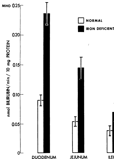
FIGURE 5 Microsomal heme oxygenase activity in the intestinal mucosa of normal and iron-deficient rats. Enzyme assays were carried out in the 20,000- g supernatant fraction of mucosa of intestinal segments obtained from four normal and eight iron-deficient rats. Results are expressed as mean \pm SEM.
