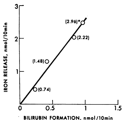
FIGURE 1 Comparison between bilirubin formation and iron release by microsomal heme oxygenase in the same 20,000- g supernatant fraction prepared from rat spleen. Each point represents the mean of four individual determinations at the indicated protein concentrations. (*) Protein concentration, milligrams per milliliter.
