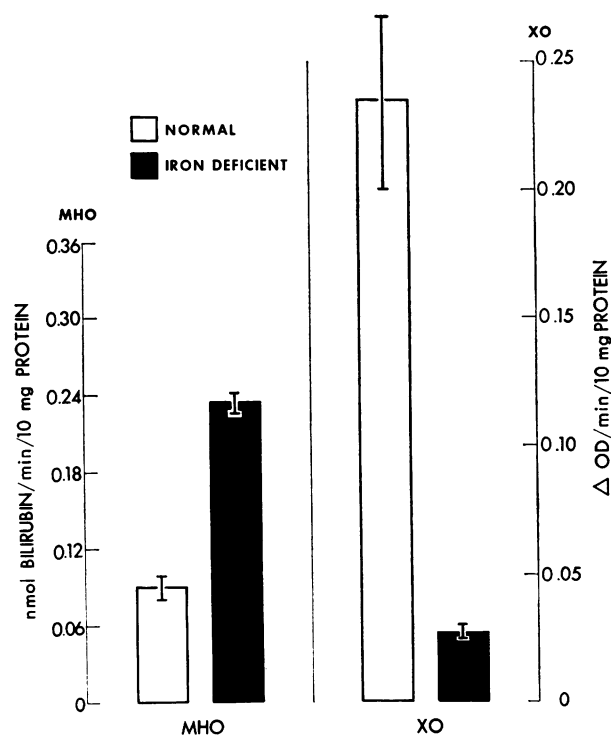
FIGURE 8 Microsomal heme oxygenase (MHO) and xanthine oxidase (XO) activity in duodenal mucosa of normal and iron-deficient rats. Enzyme assays were carried out in the 20,000- g supernatant fraction of four normal and eight iron-deficient rats. Results are expressed as mean \pm SEM.
