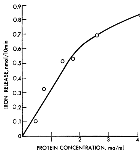
FIGURE 6 Reaction rate as a function of enzyme concentration. Heme oxygenase activity, expressed as nanomole iron released in 10 min, was measured in the 20,000- g supernatant fraction of duodenal mucosa obtained from two normal rats. Each point represents the average value of two separate determinations at the protein concentrations indicated on the abscissa.
