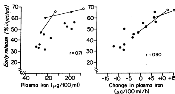
FIGURE 3 Relationship between the percent of the injected dose of ^{59}\text{Fe} DRBC released in the early phase and either the plasma iron level 3 h after injection (left) or the rate of change in plasma iron during the first 3 h of study (right). A significantly better correlation was observed when early release is related to the rate of change in plasma iron ( P < 0.001 ) than to the level of plasma iron ( P < 0.01 ). The open circles represent studies repeated in the same dog 12 h after the initial study.
