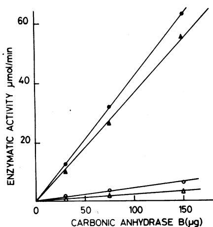
FIGURE 4 \text{CO}_2 hydration activity by purified CA B preparations at two substrate concentration (○), 0.053 M; (△), 0.025 M. (○, △), purified mutant form of CA B and (●, ▲), normal form.
