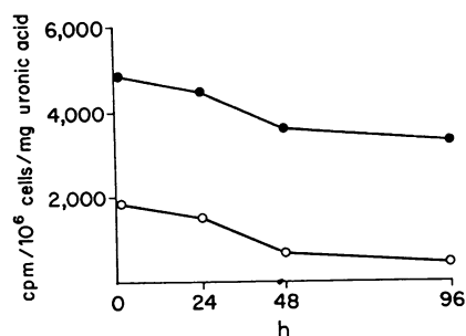
FIGURE 2 Comparison of the loss of ^{14}\text{C} -labeled CPC-precipitable material from Marfan, ●—● and control, ○—○ fibroblasts after a ^{14}\text{C} acetate pulse for 48 h.
