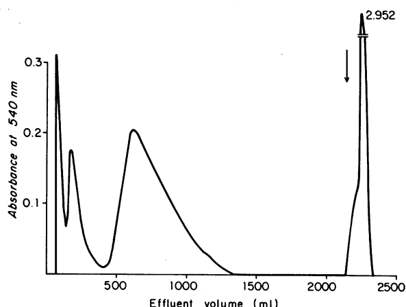
FIGURE 3 Elution profile of a hemolysate containing Hb's A and Bethesda. CG-50 Amberlite chromatography using a 2.5 \times 25 cm column at 5^{\circ}\text{C} . The flow rate was 25 ml/hr and fraction volume 8.0 ml. 430 mg of hemoglobin was applied on the column. The first three chromatographic peaks, A_s , Bethesda s , and A, were eluted with 0.1 M potassium phosphate buffer in 10^{-3} M KCN (pH 7.0). The Bethesda peak was eluted with 0.1 M potassium phosphate in 10^{-3} M KCN and 5 \times 10^{-1} M NaCl (pH 7.0).
