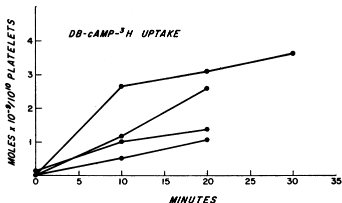
FIGURE 7 Uptake of radioactivity by platelets after incubation in citrated PRP of DB-cAMP- ^3\text{H} and 10^{-8} M carrier DB-cAMP at 37^\circ\text{C} for varying periods (four experiments). Results were corrected for trapped plasma by the use of human albumin- ^{125}\text{I} as a plasma marker (see Methods) and are expressed as nanomoles uptake of DB-cAMP per 10^{10} platelets.
