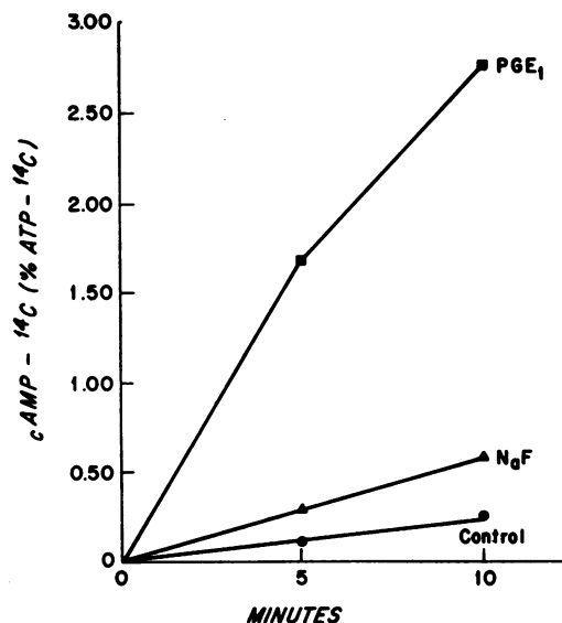
FIGURE 8 Conversion of 0.48 \times 10^{-3} M ATP- ^{14}\text{C} to cAMP- ^{14}\text{C} by adenylyl cyclase in disrupted platelets. Results are expressed as per cent conversion of substrate ATP to cAMP. Activity was stimulated by 10^{-2} M NaF or 10^{-8} M prostaglandin \text{PGE}_1 added to the platelet suspension immediately before the incubation mixture. Platelet count of original PRP 439,000/ \text{mm}^3 .
