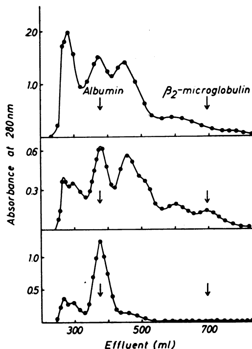
FIGURE 1 Chromatography on Sephadex G100 of concentrated proteins (329 mg) from pooled normal urine (top), of concentrated proteins (117 mg) from a patient with chronic cadmium poisoning (middle), and of concentrated proteins (146 mg) from a patient with glomerulonephritis (bottom). The column (2.9 × 133.5 cm) was equilibrated with 0.1 M Tris-HCl buffer, pH 8.0, containing 1.0 M NaCl. Fractions of 5 ml were collected at a flow rate of 15 ml/hr. The distribution in the effluent of albumin and \beta_2 -microglobulin was determined by a single radial immunodiffusion technique. The position of the maximum concentrations of the two proteins are indicated by arrows.
