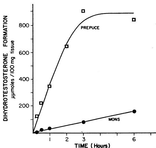
FIGURE 5 Time course of dihydrotestosterone- 3 H formation by slices of prepuce and mons. Tissue slices (100 mg) obtained from different sites in different patients were incubated for varying periods of time as described in Fig. 1. The radioactive steroids were then separated and analyzed for radioactivity as described in the text.
