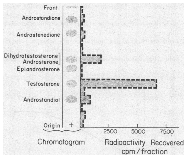
FIGURE 1 Comparison by gas-liquid and thin-layer chromatography of the metabolites of testosterone-1,2- ^3\text{H} after incubation with slices of prepuce. Slices of prepuce obtained from a newborn infant (100 mg) were incubated with testosterone-1,2- ^3\text{H} ( 9.5 \times 10^{-7} mole/liter), glucose ( 1.1 \times 10^{-3} mole/liter), penicillin (2500 U), and Krebs-Ringer phosphate buffer, pH 7.4, in a total volume of 2.5 ml. After incubation for 1 hr at 37°C, the mixture was saponified, and the steroids were extracted into chloroform:methanol and backwashed as described in the text. Aliquots of the chloroform:methanol extracts and appropriate mixtures of steroid standards were chromatographed either by thin-layer chromatography or by gas-liquid chromatography, and the thin-layer scrapings and gas eluates were then assayed for radioactivity.
