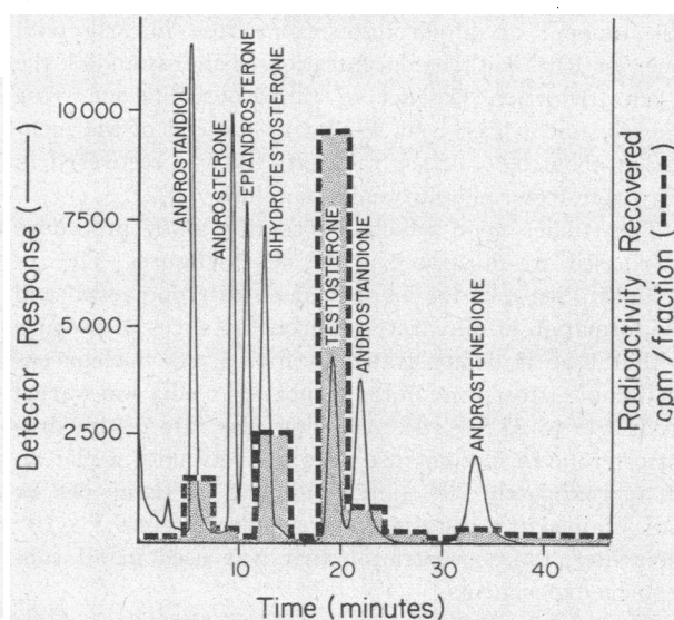
FIGURE 1 Comparison by gas-liquid and thin-layer chromatography of the metabolites of testosterone-1,2- ^3\text{H} after incubation with slices of prepuce. Slices of prepuce obtained from a newborn infant (100 mg) were incubated with testosterone-1,2- ^3\text{H} ( 9.5 \times 10^{-7} mole/liter), glucose ( 1.1 \times 10^{-3} mole/liter), penicillin (2500 U), and Krebs-Ringer phosphate buffer, pH 7.4, in a total volume of 2.5 ml. After incubation for 1 hr at 37°C, the mixture was saponified, and the steroids were extracted into chloroform:methanol and backwashed as described in the text. Aliquots of the chloroform:methanol extracts and appropriate mixtures of steroid standards were chromatographed either by thin-layer chromatography or by gas-liquid chromatography, and the thin-layer scrapings and gas eluates were then assayed for radioactivity.
