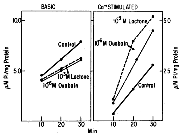
FIGURE 5 Effect of ouabain and alpha angelica lactone on phosphate released from ATP in the presence and absence of calcium. Microsomes (0.1 mg/cc) were incubated at 25^\circ\text{C} in the presence of 4 mM MgATP, 8 mM histidine, 0.12 M KCl, in the presence and absence of 10^{-4} M \text{CaCl}_2 with ouabain and alpha angelica lactone as shown. Samples were taken at 10, 20, and 30 min. Left panel shows released inorganic phosphorus ( \text{P}_i ) in absence of \text{Ca}^{++} ; right panel is additional \text{P}_i released in the presence of \text{Ca}^{++} . (Curves fail to go through the ordinate at zero because blanks were not subtracted.)
