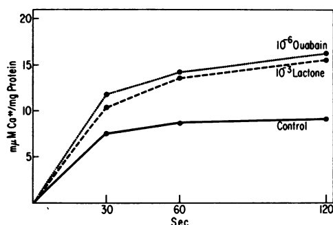
FIGURE 1 Calcium turnover measured by dilution of 45 Ca ++ with unlabeled Ca ++ . Microsomes (0.2 mg of protein per cc) were incubated in the presence of 5 mM adenosine triphosphate (ATP), 10 mM histidine, 0.12 M KCl, and 2.5 × 10 -6 M 45 CaCl 2 for 5 min at 25°C. At time zero 150 mμmoles of CaCl 2 are added, and the change in bound 45 Ca ++ is measured at intervals shown. Abbreviations: lactone, alpha angelica lactone.
