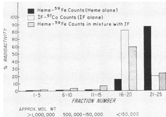
FIGURE 3 Sucrose density gradient ultracentrifugation patterns of heme- ^{59}\text{Fe} and IF- ^{57}\text{Co} interaction.
