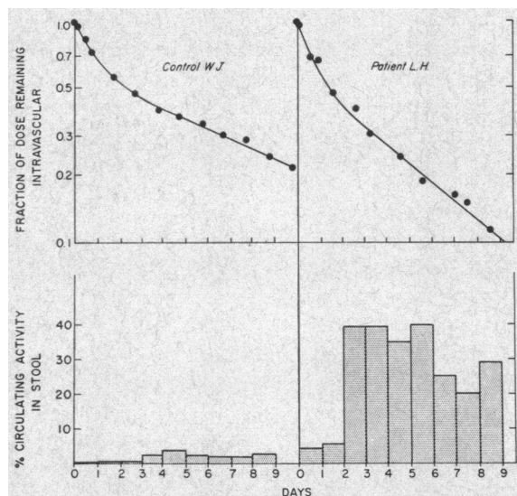
FIG. 3. TURNOVER OF INTRAVENOUSLY ADMINISTERED CERULOPLASMIN- 67 CU IN MAN. The radioactivity remaining in the plasma and the fecal clearance of 67 Cu for a control subject (W.J.) and a patient with intestinal lymphangiectasia (L.H.) are shown. The patient has a shorter ceruloplasmin- 67 Cu survival and a markedly increased fecal clearance of 67 Cu from the plasma.
