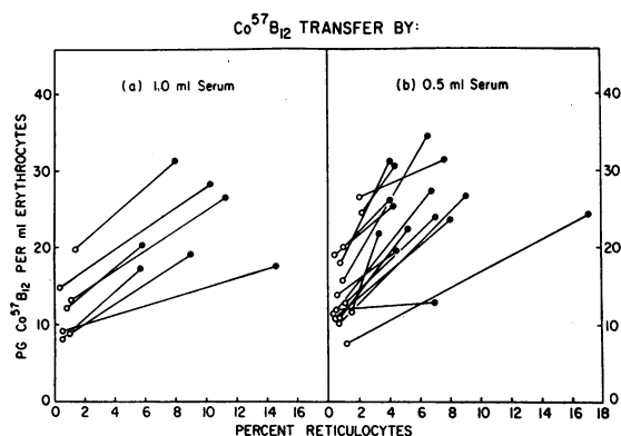
FIG. 1. SERUM-MEDIATED B_{12} - ^{57}\text{Co} UPTAKE BY ERYTHROCYTES. The increased amount (in picograms) of B_{12} - ^{57}\text{Co} transferred to reticulocyte-rich (closed circles) over reticulocyte-poor (open circles) suspensions of erythrocytes, in the same experiments, is shown by connected points.
