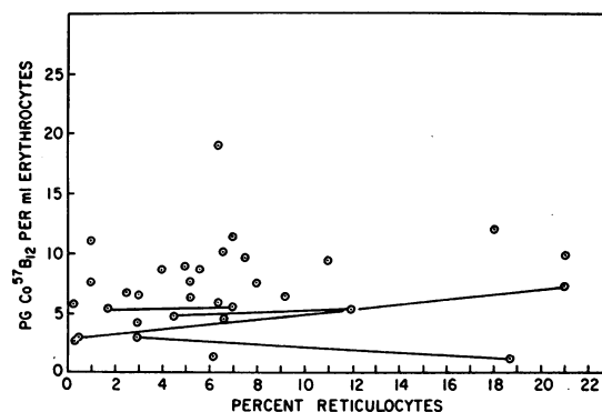
FIG. 2. SALINE-MEDIATED B_{12} - ^{57}\text{Co} UPTAKE BY ERYTHROCYTES. The amount of B_{12} - ^{57}\text{Co} taken up by reticulocyte-rich suspensions of erythrocytes is less from saline than serum (compare with Figure 1). Where tested in the same experiment there was no difference in the uptake of B_{12} - ^{57}\text{Co} by reticulocyte-rich as compared to reticulocyte-poor suspensions of erythrocytes (connected points).
