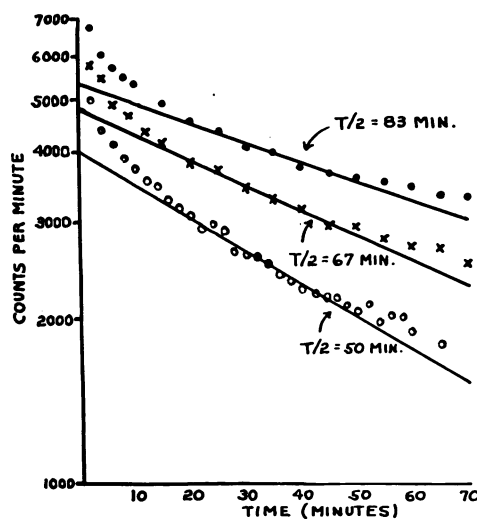
FIG. 1. THREE ILLUSTRATIVE CURVES PLOTTED ON SEMI-LOG PAPER SHOWING THE REGRESSION OF NET COUNTS PER MINUTE ON TIME AFTER INTRAVENOUS INJECTION OF I^{131} -L-THYROXINE. THE HALF-TIME VALUE IS DERIVED FROM CALCULATION OF THE SLOPE OF THAT SEGMENT OF THE CURVE BETWEEN 20 AND 50 MINUTES.
