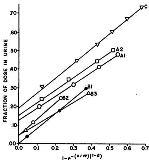
FIG. 2. THE FRACTION OF THE DOSE OF LABELED UREA RECOVERED IN THE URINE PLOTTED AGAINST A TIME INTEGRAL WHICH REPRESENTS THE FRACTION ANTICIPATED FROM THE PLASMA DISAPPEARANCE
