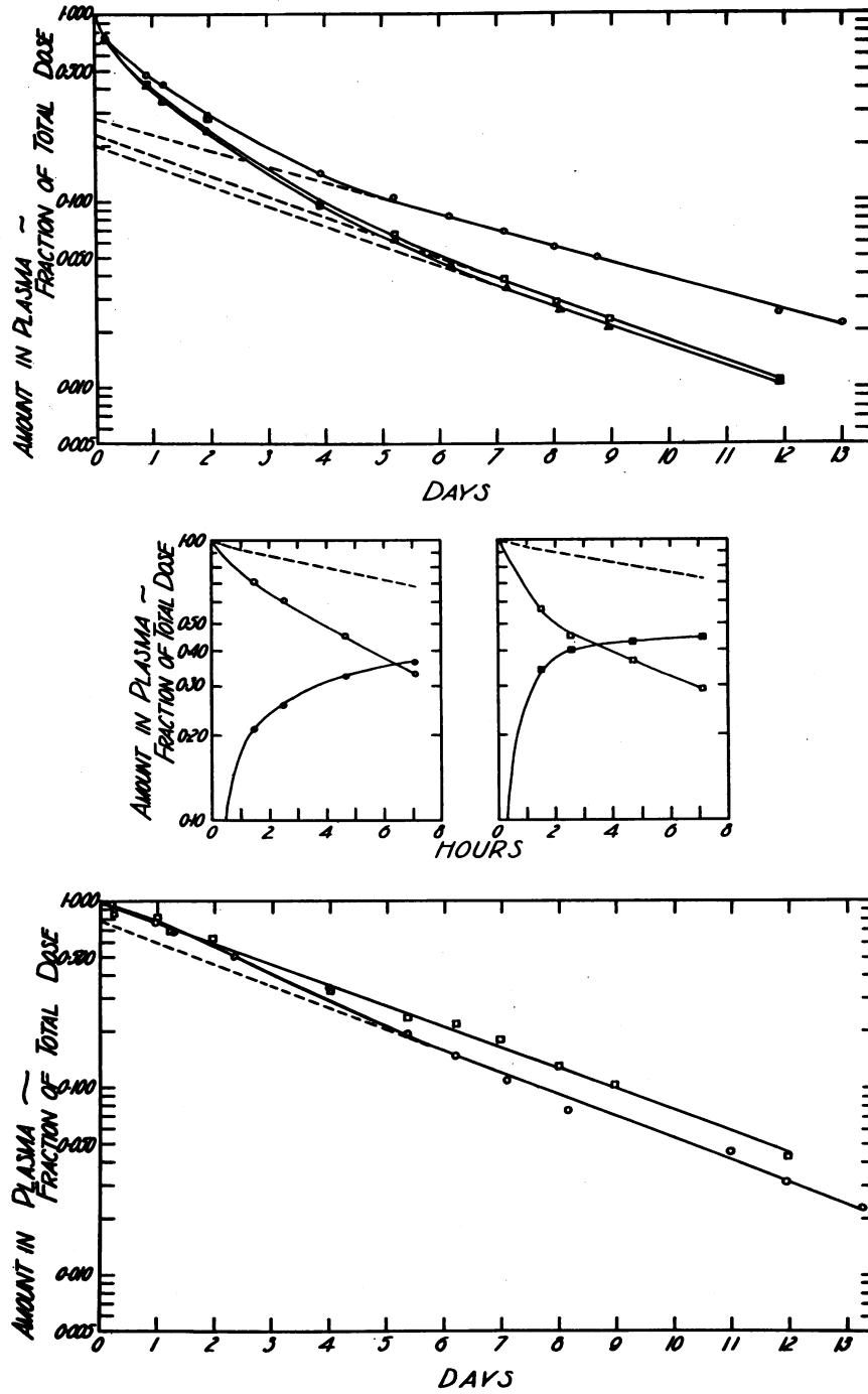
FIG. 3. THE DISAPPEARANCE OF RADIOACTIVITY FROM THE CIRCULATION AFTER INTRAVENOUS INJECTION OF IODINATED "NORMAL" LOW DENSITY LIPOPROTEINS Upper chart, total plasma radioactivity in normal adults: □ J. B. △ R. B. ○ E. S. Middle charts: W. H. D. C. Total plasma radioactivity --- --- Low density lipoproteins ○ □ S 1 3 to 9 lipoproteins ● ■ Lower chart, total plasma radioactivity in nephrotic children: ○ J. G. □ D. O.
